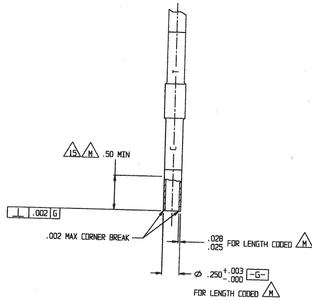
VIEW F FOR -1 ROTATED 7°30' COUNTERCLOCKWISE SCALE 2/1
