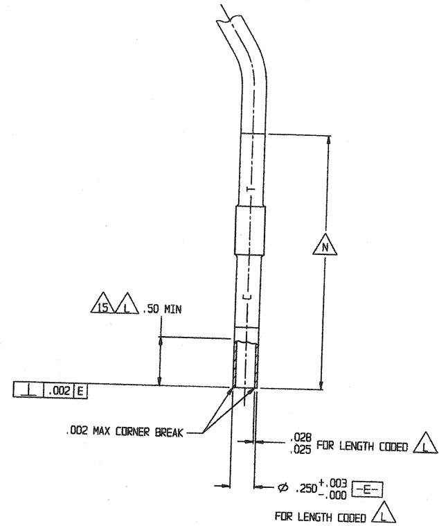
VIEW D SHEET 1 FOR -1 SCALE 2/1
