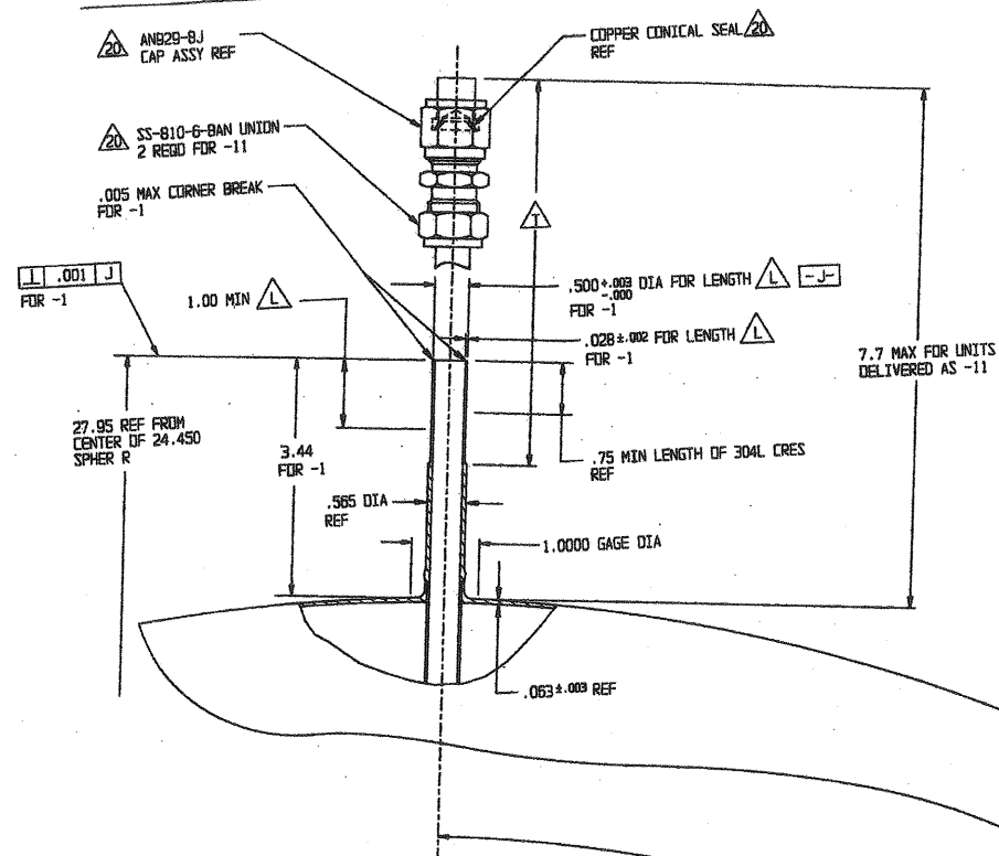
SECTION D-D SHEET 1 SCALE: 1/1
