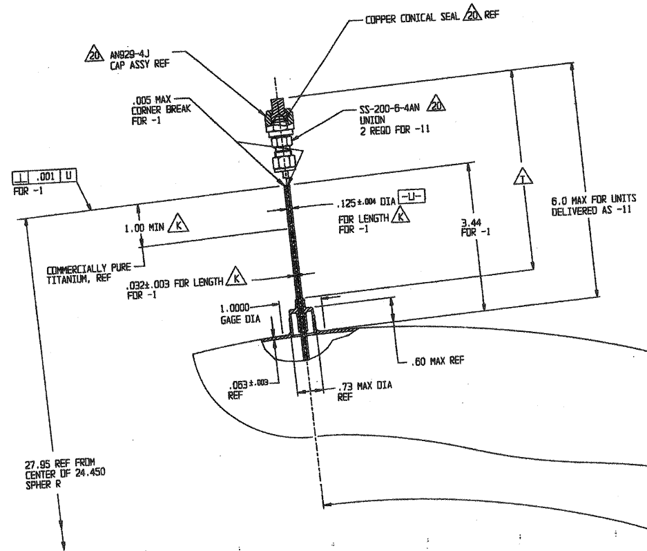
SECTION G-G SHEET 1 SCALE: 1/1 TYP 2 PLACES
