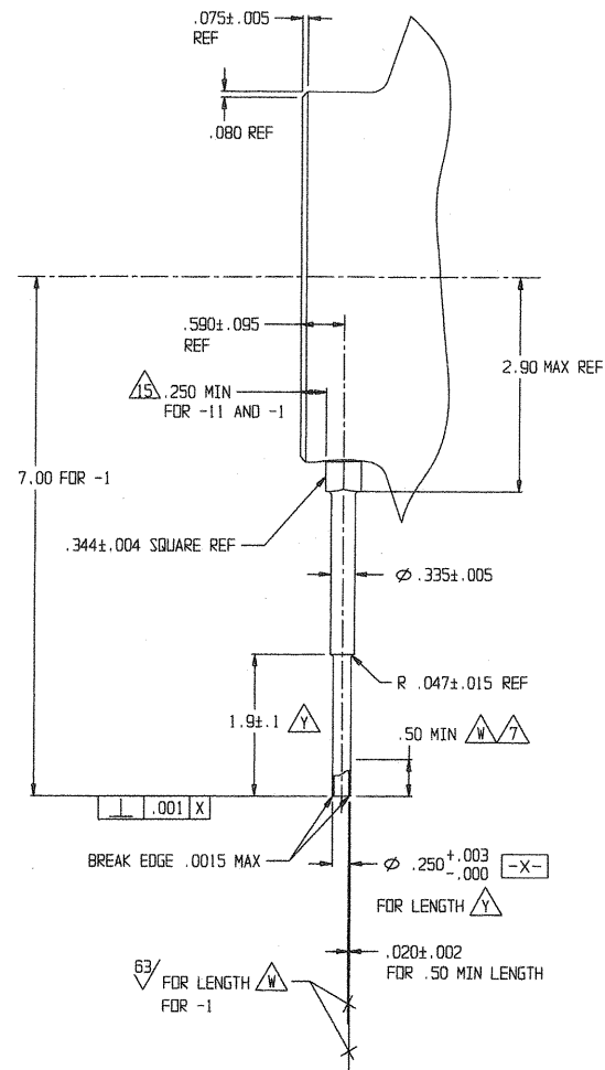
VIEW H SHEET 1 SCALE 1/1
